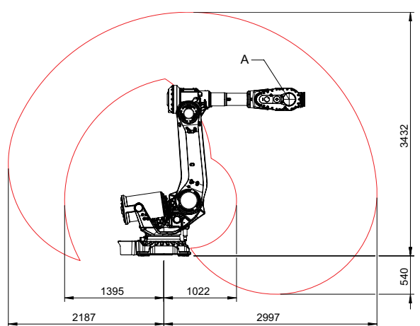
Working range IRB 6740-260/3.0
