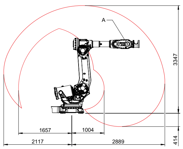
Working range IRB 6730-220/2.9 LID
